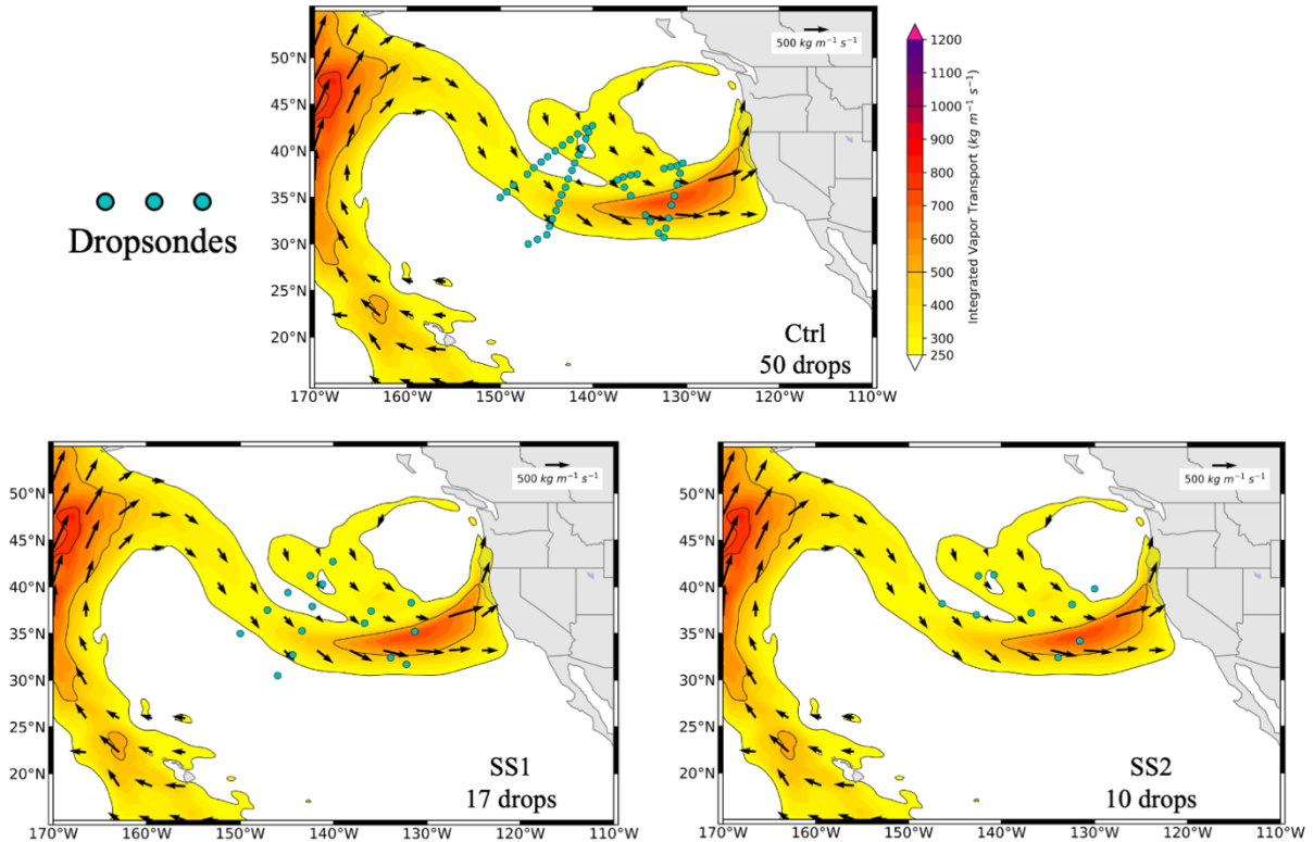
Figure Caption: The ERA-5 integrated vapor transport (shades and vectors, [\text{kg m}^{-1} \text{s}^{-1}] ) and locations of dropsondes (Aqua markers) assimilated in three experiments for analysis valid at 0000 UTC 27 Jan 2021. Top: in the Ctrl experiment; Bottom left: in the SS1 experiment, Bottom right: in the SS2 experiment. The dropsondes are collected from two C-130 aircraft during AR Recon 2021 IOP7.
