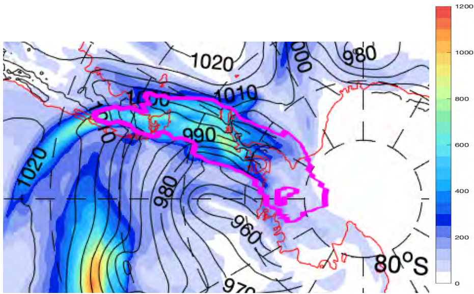
Figure: Integrated water vapour transport (colors, \text{kg m}^{-1} \text{s}^{-1} ) and mean sea level pressure (contours, hPa) on 8 February 2022, 00 UTC, based on ERA5 reanalysis. The magenta contour depicts the AR shape based on Wille et al (2021) vIVT AR-tracking algorithm.
