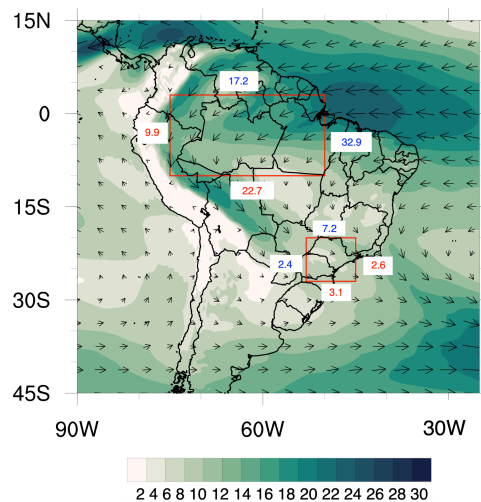
Figure 1- Climatological vertically integrated moisture flow ( \text{kg m}^{-1} \text{ s}^{-1} ) for 1979-2015 period.
