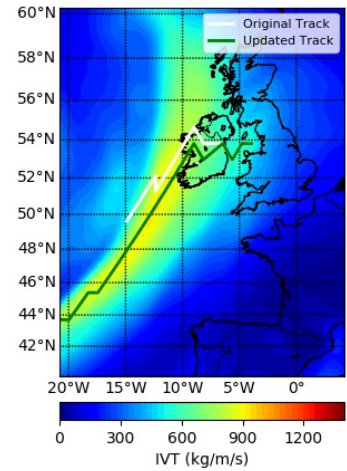
IVT Plot and AR Tracks: 20131220_15UTC
