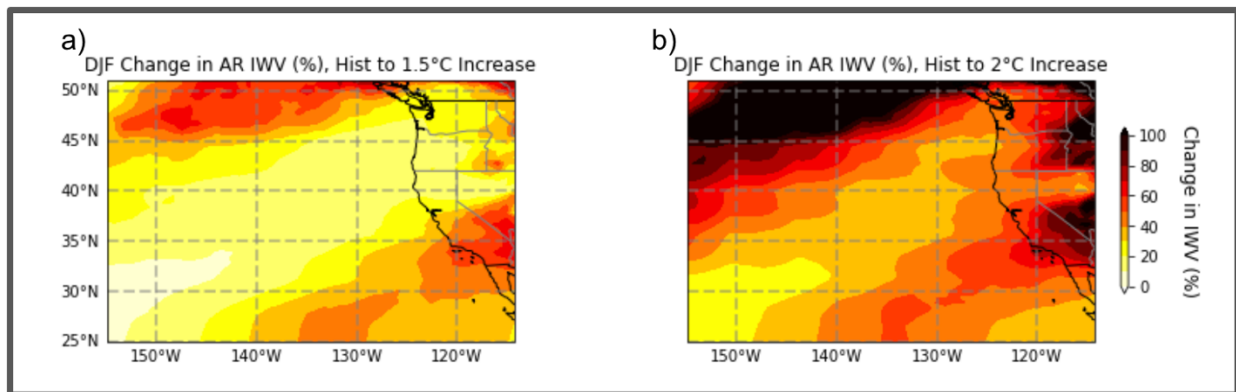
Figure: The mean percentage change in AR IWV from the a) Hist to 1.5°C increase scenario and b) Hist to 2° increase scenario during winter months
