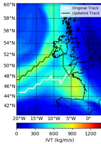
IVT Plot and AR Tracks: 20140124_13UTC
